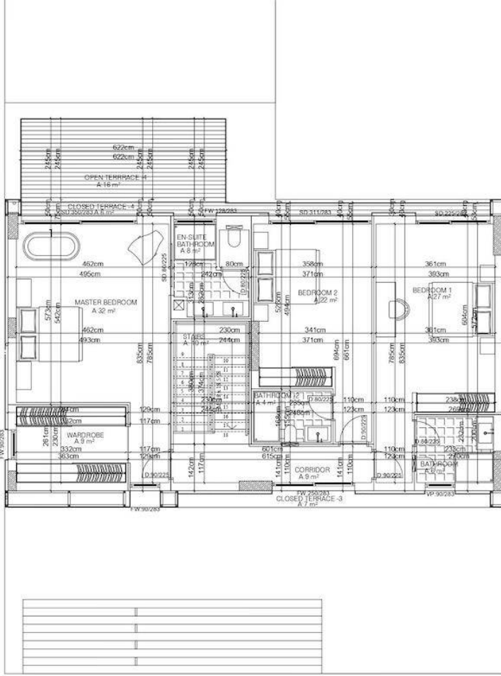
TYPE E-1. FLOOR PLAN
